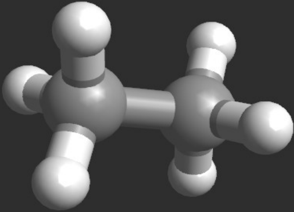
ETHANE
